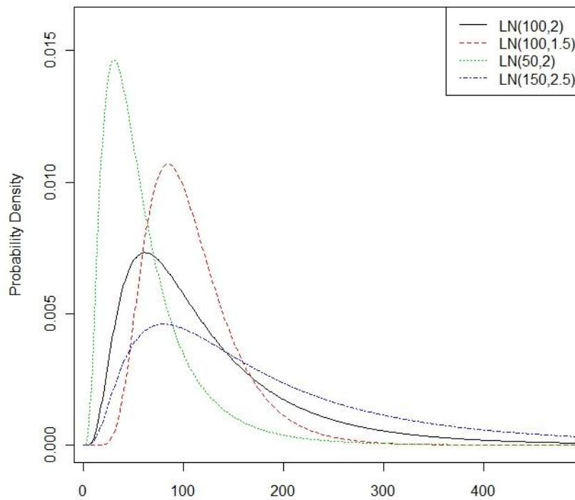
Figure 2. Examples of lognormal probability density functions
